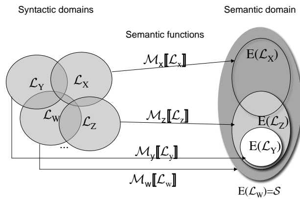
Fig. 6. Comparing expressiveness
