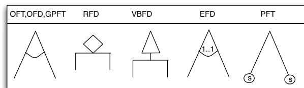
Fig. 2. Concrete syntaxes for xor -decomposition
