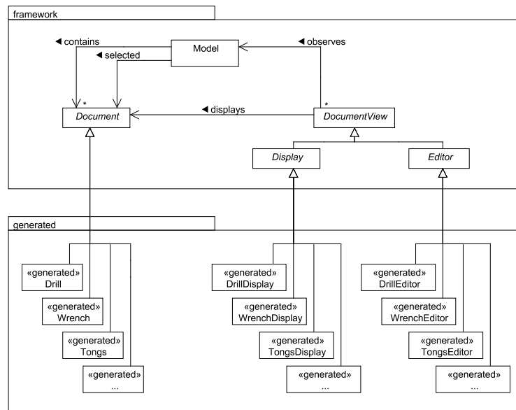
Fig. 5. Framework architecture
